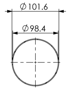
BOLLARD DETAIL SECTION/PLAN
